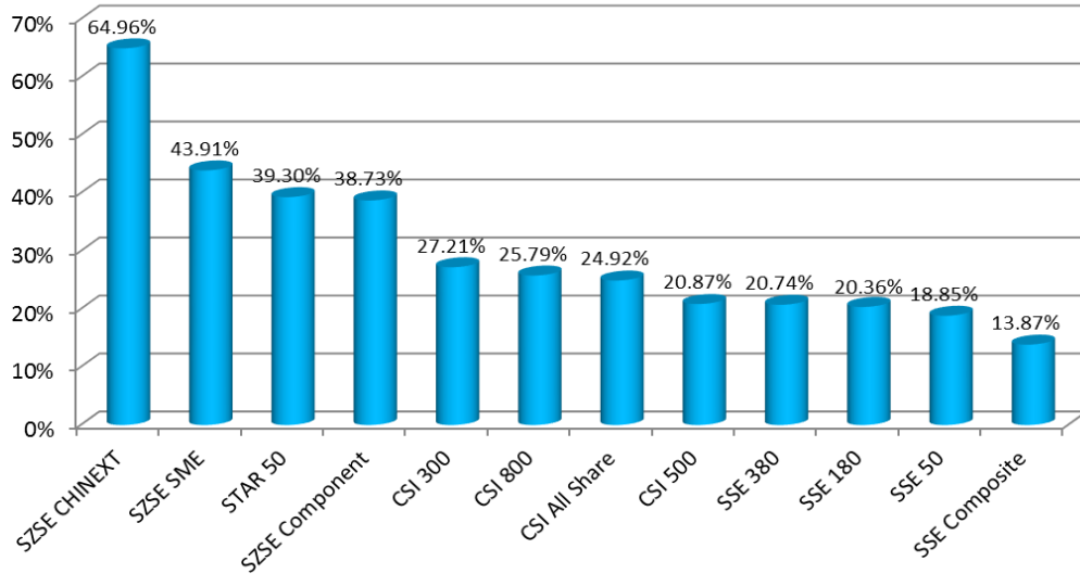
Primary Indices Performance
