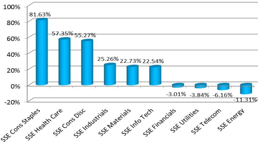
Performance of SSE Sector Indices
